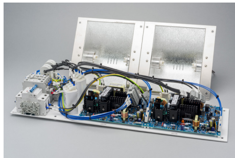
UV Light Banks • For DC's with single solution configuration
