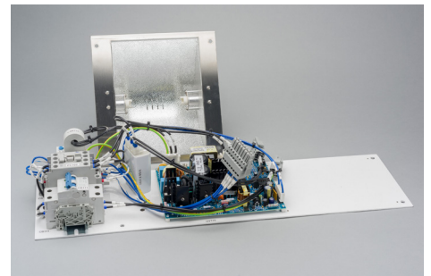
UV Light Banks • For DC's with dual solution configuration
