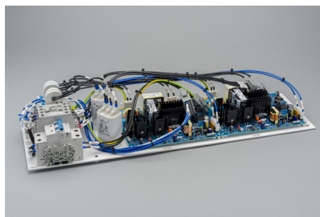
Electrical Light Bank Panel
